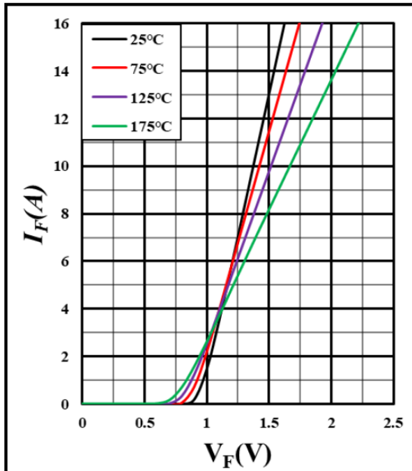
Figure 1. Forward characteristics
